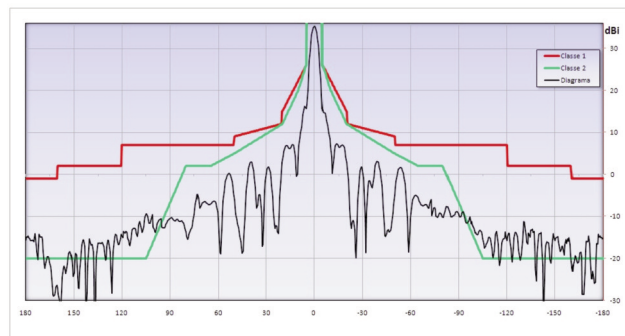
Diagrama Horizontal
