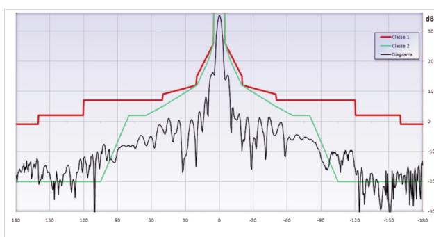
Diagrama Horizontal
